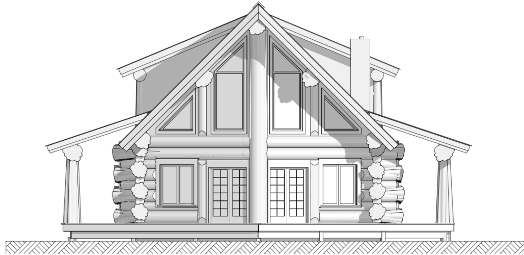
FRONT
